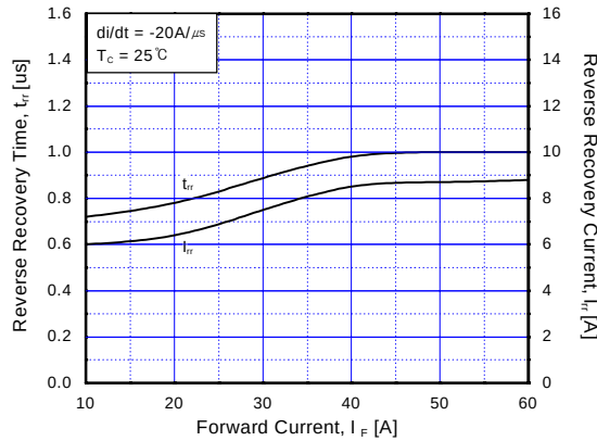
Fig 15. Reverse Recovery Characteristics vs. Forward Current
