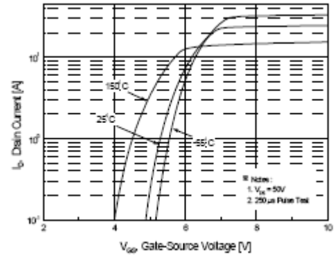
Fig.2 Transfer Current Characteristics
