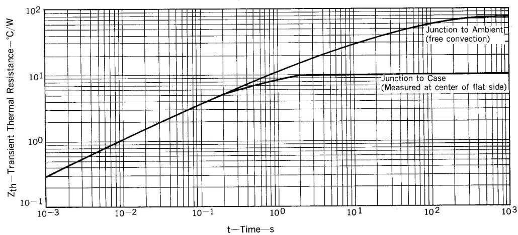
Fig. 11 Z_{th} CHARACTERISTICS
