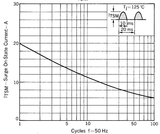
Fig. 10 I_{TSM} RATINGS
